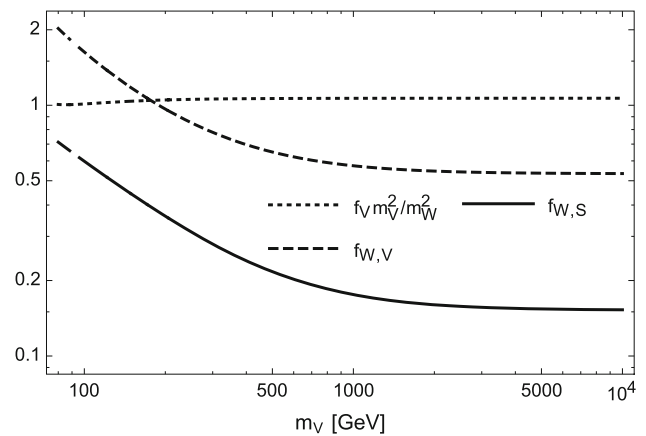
Fig. 3 f_V m_V^2 / m_W^2, f_{W,S} and f_{W,V} as functions of the SU(2)_R scale m_V
